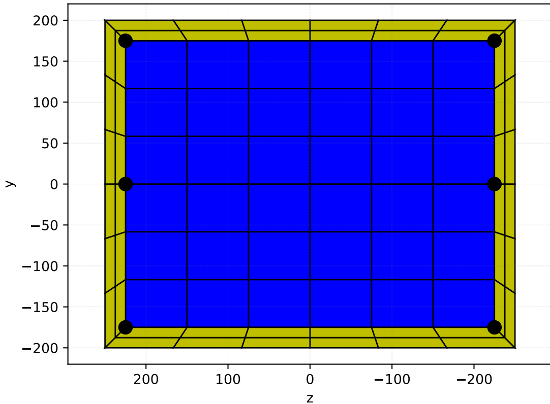
Beam Section for Staging
